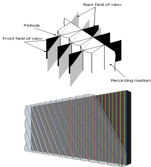
Fig.1 Lenticular sheet model in integral ray tracer
