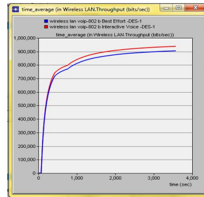
Figure 5: The throughput (bps) for IEEE 802.11b with best effort and interactive voice services
