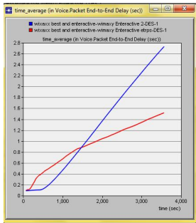
Figure 16: Packet end-to-end delay (sec) for WiMax UGS and ertPS with interactive service
