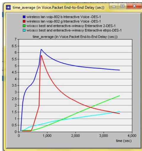
Figure 24: Voice packet end-to-end delay on Wi-Fi and WiMAX networks with interactive service
