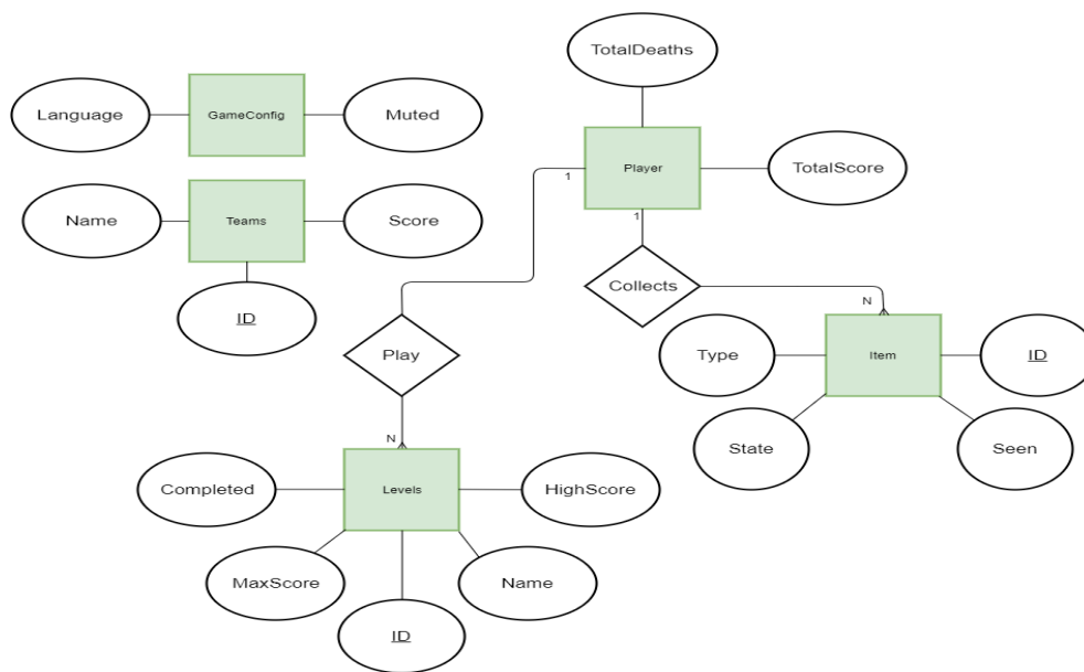
Figure 10: game ERD
