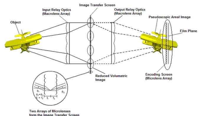
Figure 1: An advanced Integral Imaging system [96].
