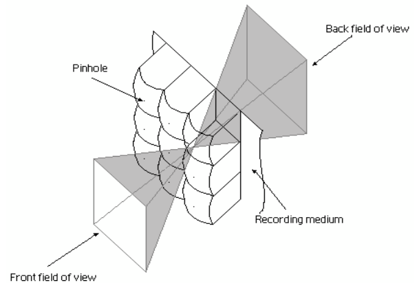
Figure 3: Micro-lens array in integral ray tracing.
