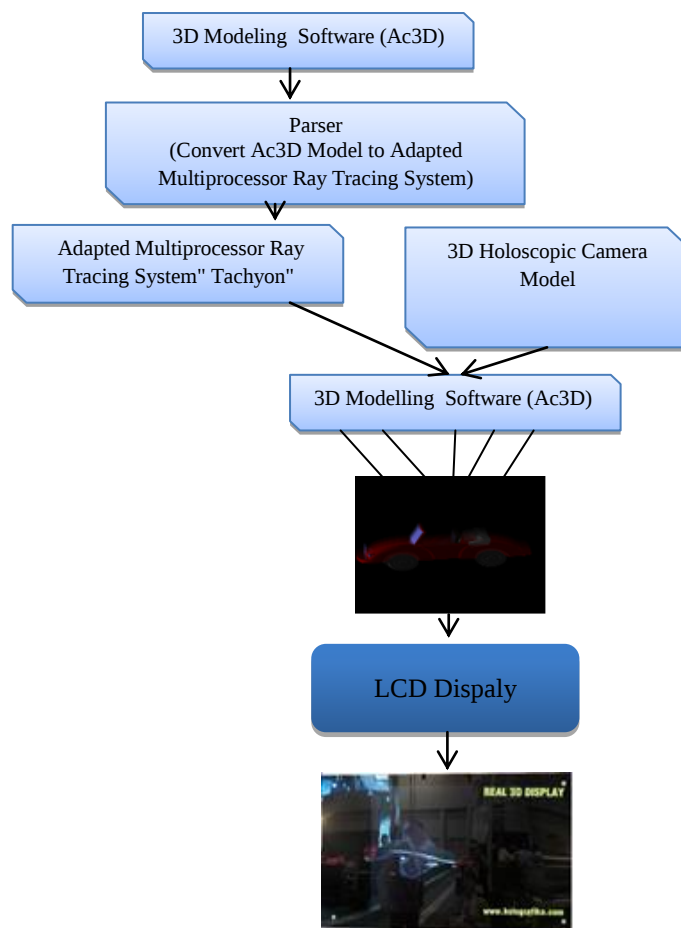
Figure 5: 3D Integral Images content parser modules diagram.
