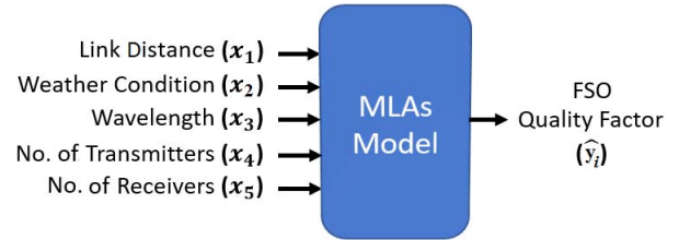
Fig. 1. Machine learning block diagram.
