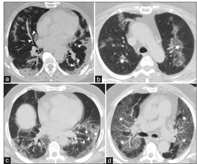
Figure 3: Axial noncontrast chest computed tomography of other features of coronavirus disease 2019 observed in this study. (a) Subpleural traction bands with architectural distortion (arrowheads), and bronchial wall thickening (arrowheads); (b) Nonperipheral patches of ground-glass opacity (stars); (c) Vessel dilatation (arrowheads) within ground-glass opacity (star); (d) Extensive ground-glass opacity and consolidation (ARDS (Acute Respiratory Distress Syndrome) like) (stars)
