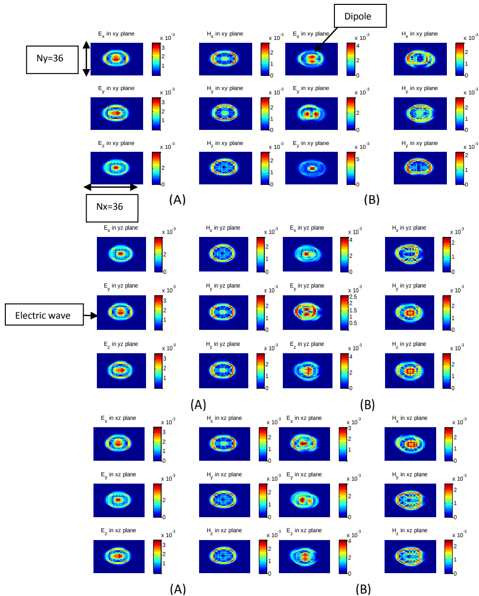
Figure 4 shows 3D FDTD simulation: slice 2 mapping of the electric (V/m) and magnetic fields (A/m) in the x-y, y-z and x-z planes after excitation. Three sources located in the same location (A) and also placed in three locations (B).
