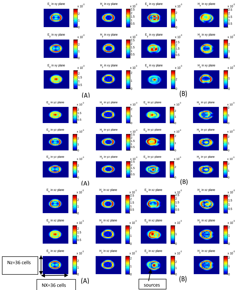
Figure 5: shows 3D FDTD simulation: slice 3 mapping of the electric (V/m) and magnetic fields (A/m) in the x-y, y-z and x-z planes Three sources located in the same location (A) and also placed in three locations (B).
