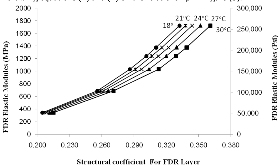
Figure 3: the relationship between the FDR modulus and the FDR layer structural coefficient for different MAATs
