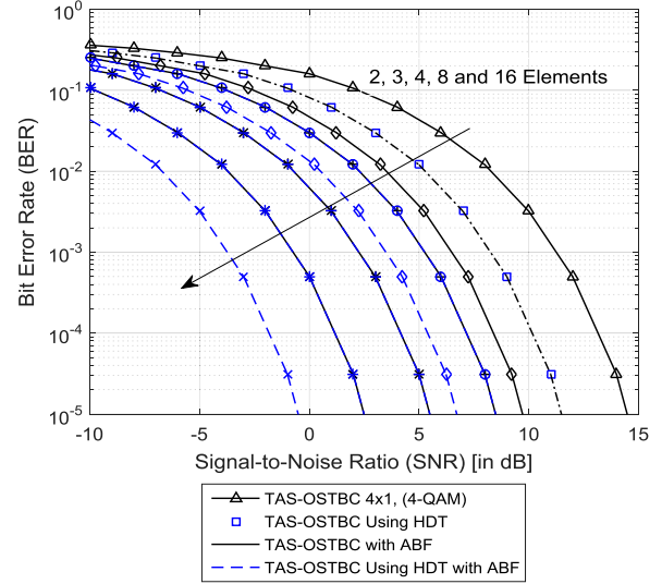
Figure 4. BER performance of TAS-OSTBC employing 4-QAM and 4 transmit antennas with analog beamforming and Hadamard transform.
