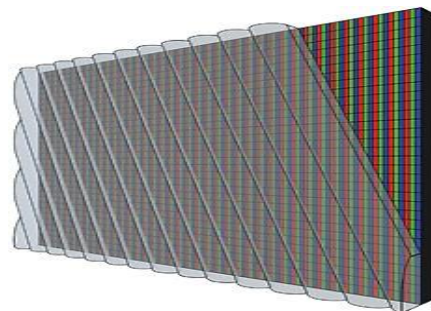
Figure 6: The Slanted arrangement of the lenticular lens and pixels in the multiview auto-stereoscopic displays.
