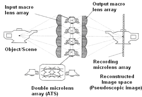
Figure 4: An advanced Integral Imaging system [96].
