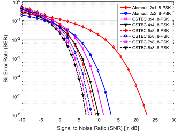
Figure 2. BER performance of Alamouti and OSTBC schemes with multiple transmit antennas employing 8-PSK over Rician fading channel with K = 10dB .
