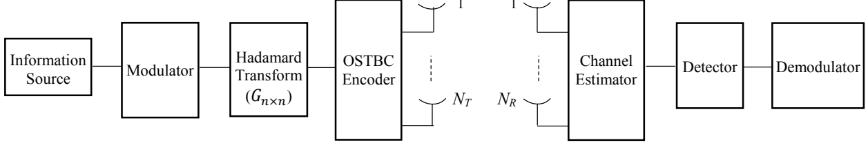
Figure 1. System model of OSTBC schemes with multiple transmit antennas using Hadamard transform.
