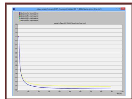
Figure.10 Media Access Delay for each end device (average)
