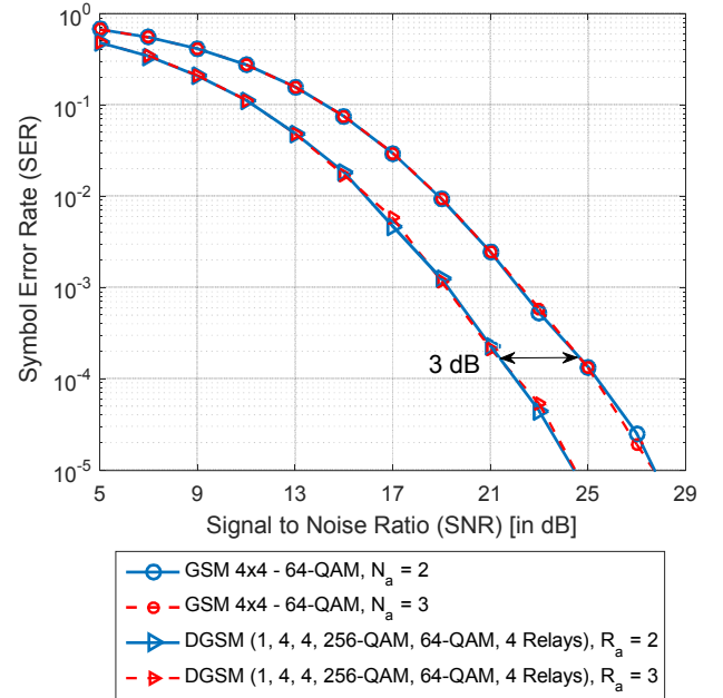
Fig. 6. SER performance of DGSM schemes (Arrow marker) compared to GSM (Circle marker) for the same modulation order, and with 2 active relays/antennas (Solid lines) and 3 active relays/antennas (Dashed lines).
